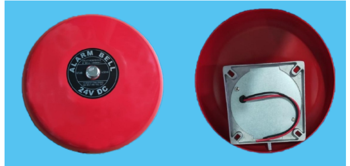
FIRE ALARM BELL Model FACB-8
